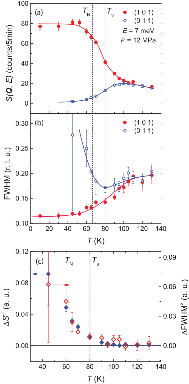
FIG. 3: Temperature dependence of (a) S(\mathbf{Q}, E) and (b) FWHM at (1 0 1) and (0 1 1) at 7 meV and 12 MPa. (c) Temperature dependence of \Delta S^{-1} (blue solid diamonds) and \Delta FWHM^2 (red open diamonds) as defined in the main text. The solid lines are guided to the eye. The vertical dashed lines indicate T_s and T_N .
